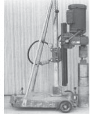
Core Test (A23.2-14C)
